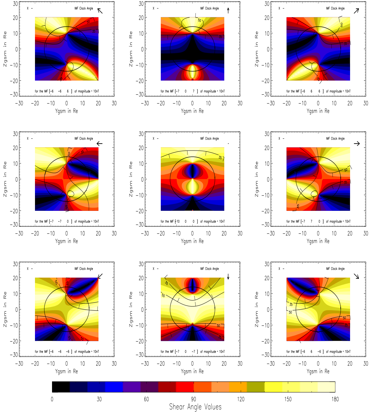
Figure 3.6: Magnetopause shears with thresholds over -X
