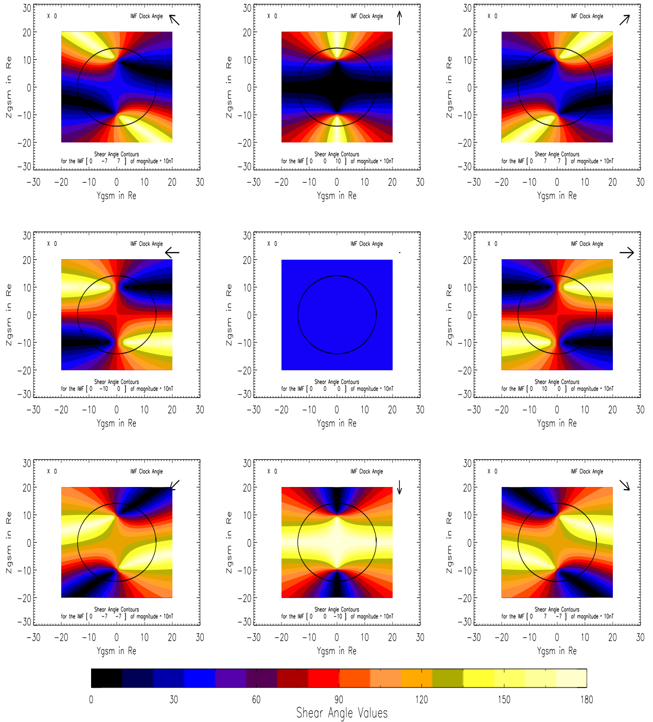
Figure 3.2: Magnetopause shears 0X
