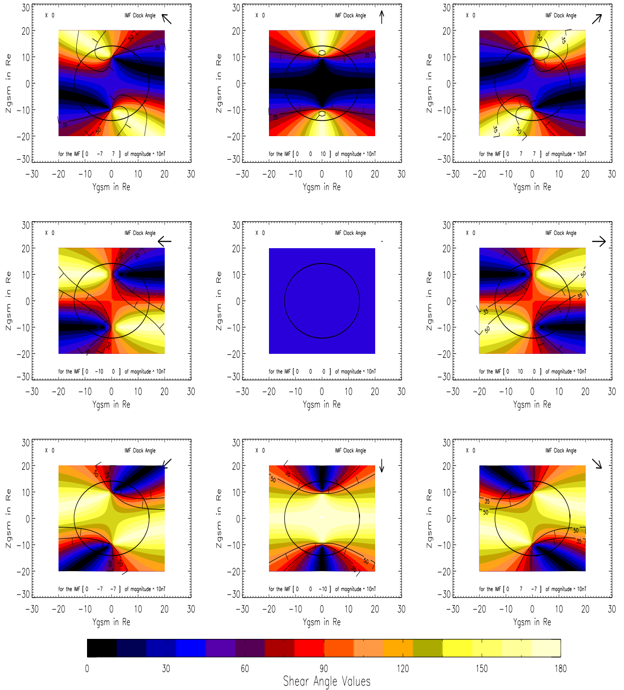
Figure 3.5: Magnetopause shears with thresholds over OX
