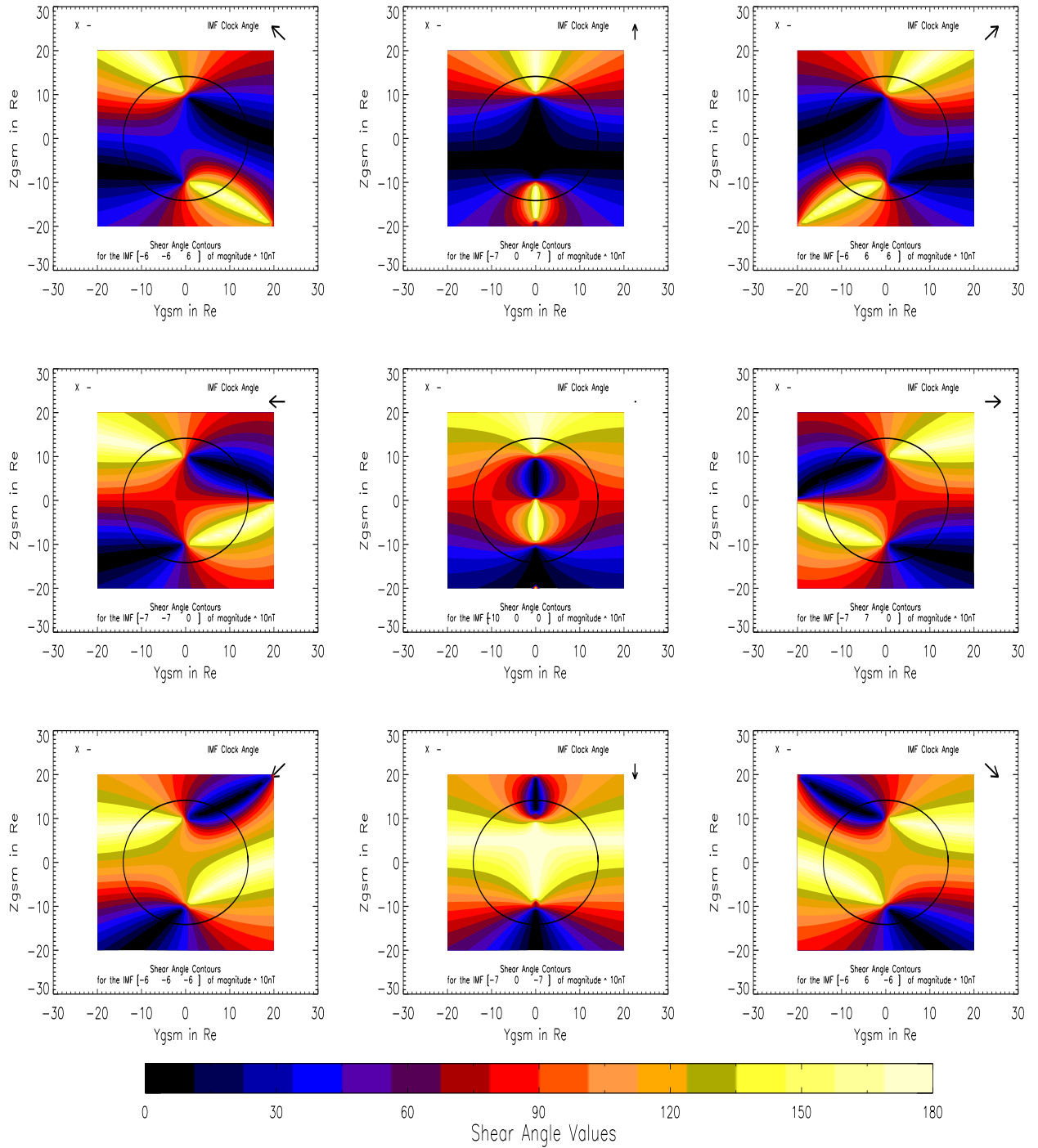
Figure 3.3: Magnetopause shears -X
