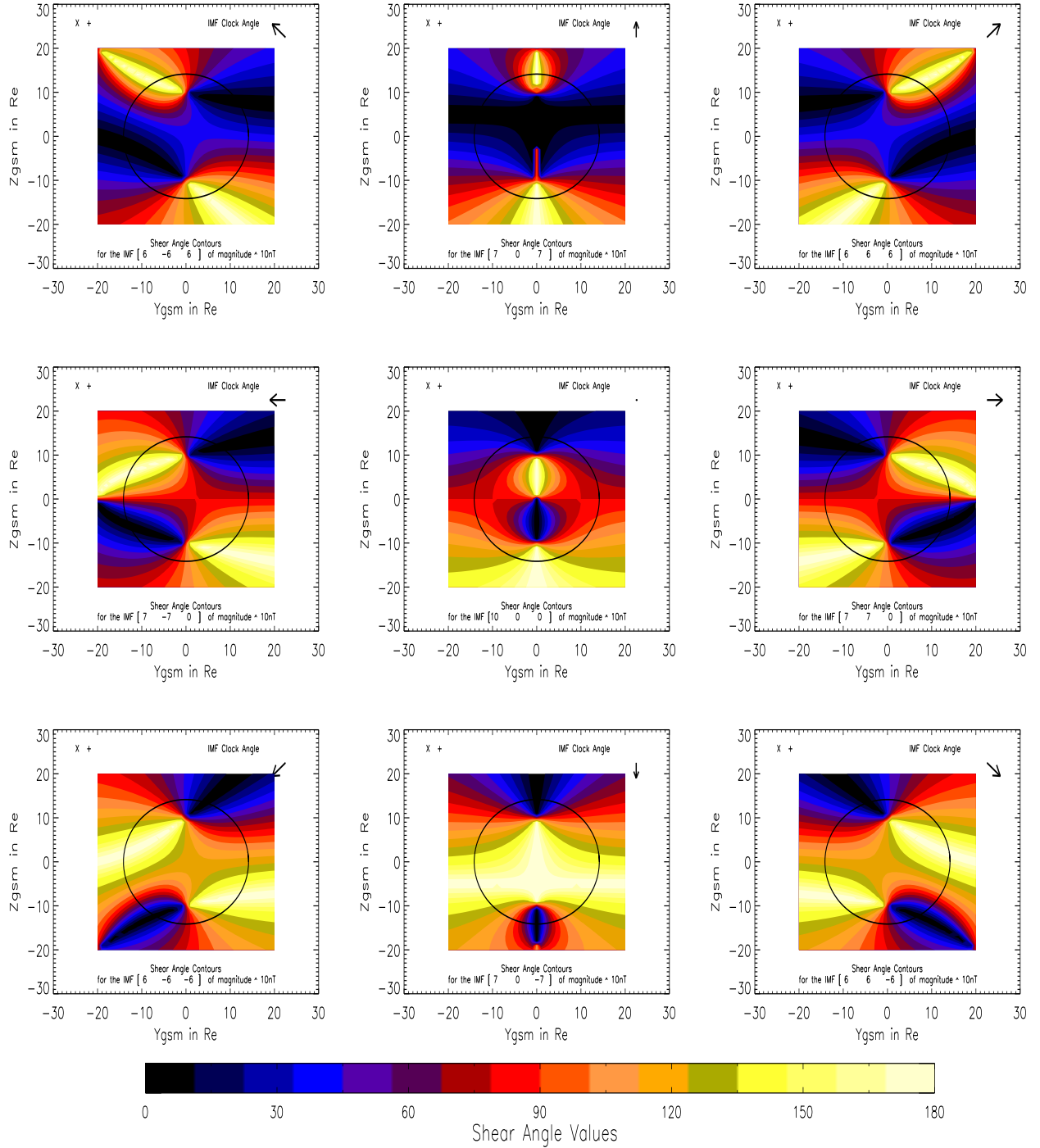
Figure 3.1: Magnetopause shears +X
