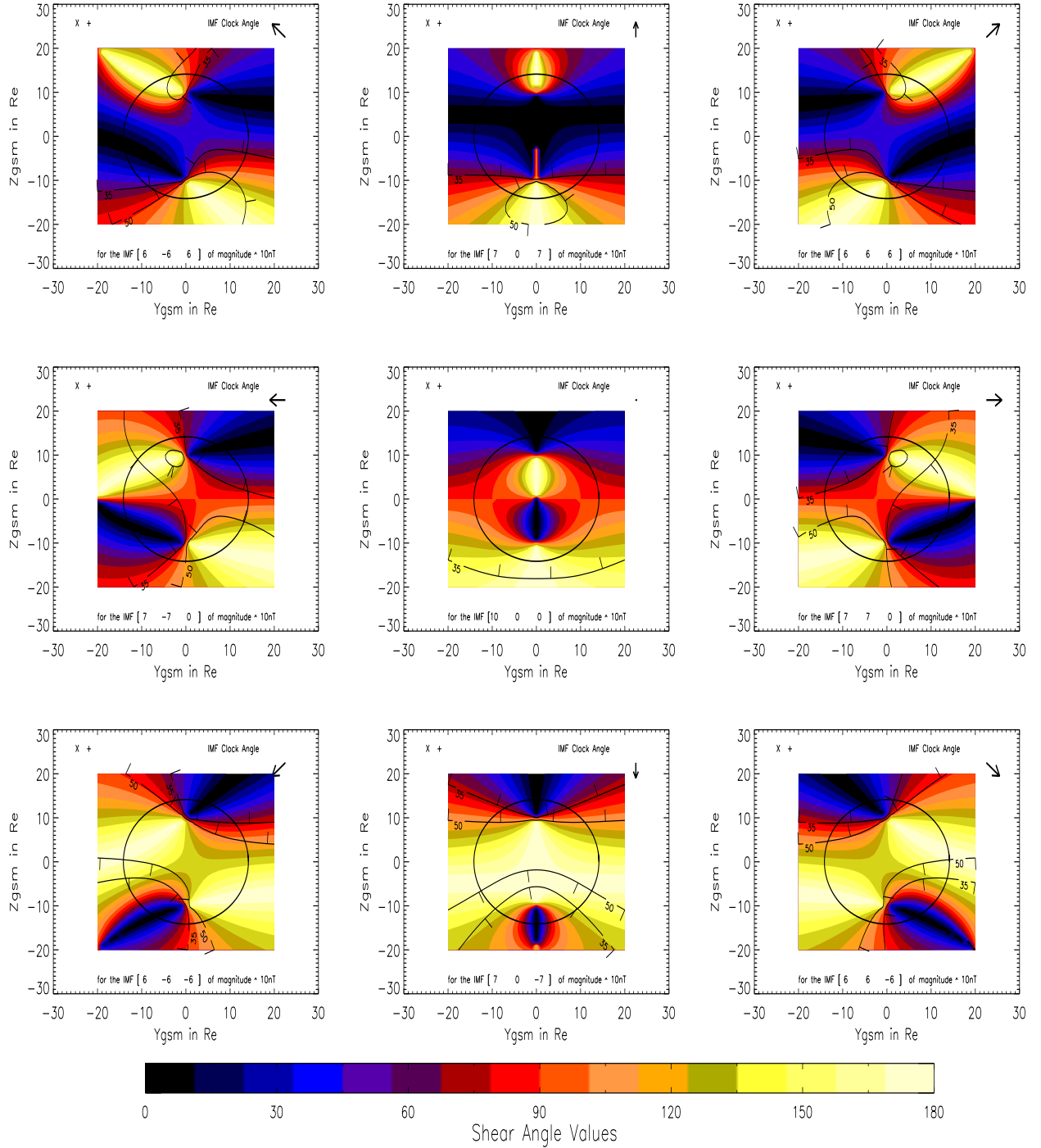
Figure 3.4: Magnetopause shears with thresholds over +X
