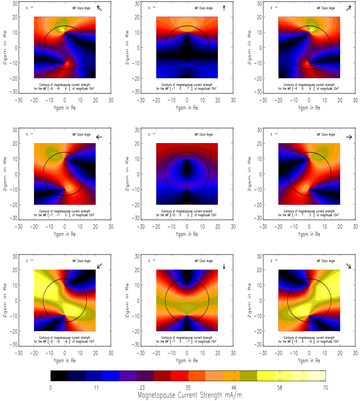
Figure 2.6: Magnetopause current strength contours -X
