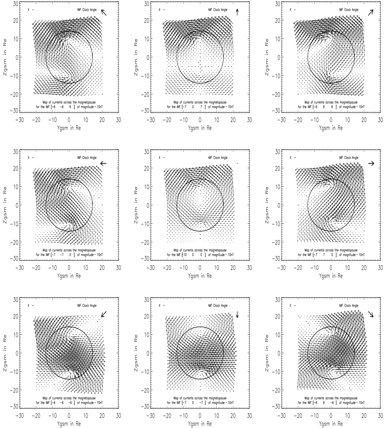
Figure 2.3: Magnetopause current -X
