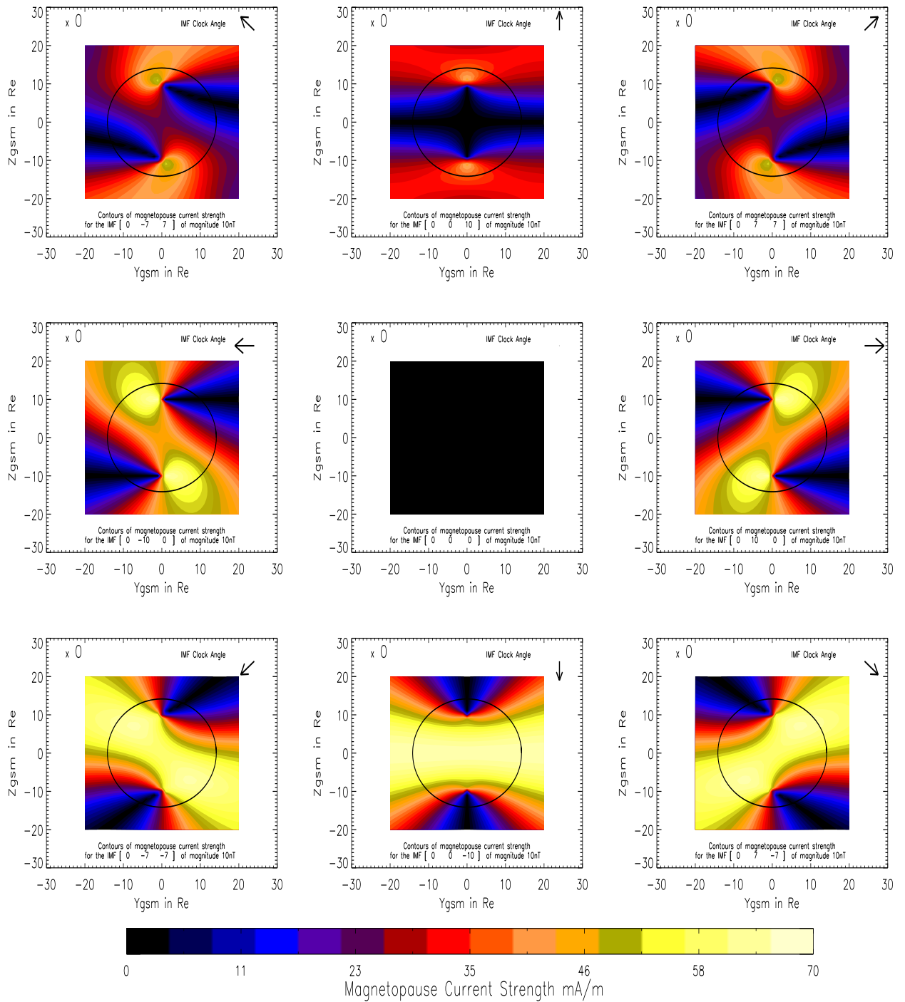
Figure 2.5: Magnetopause current strength contours 0X
