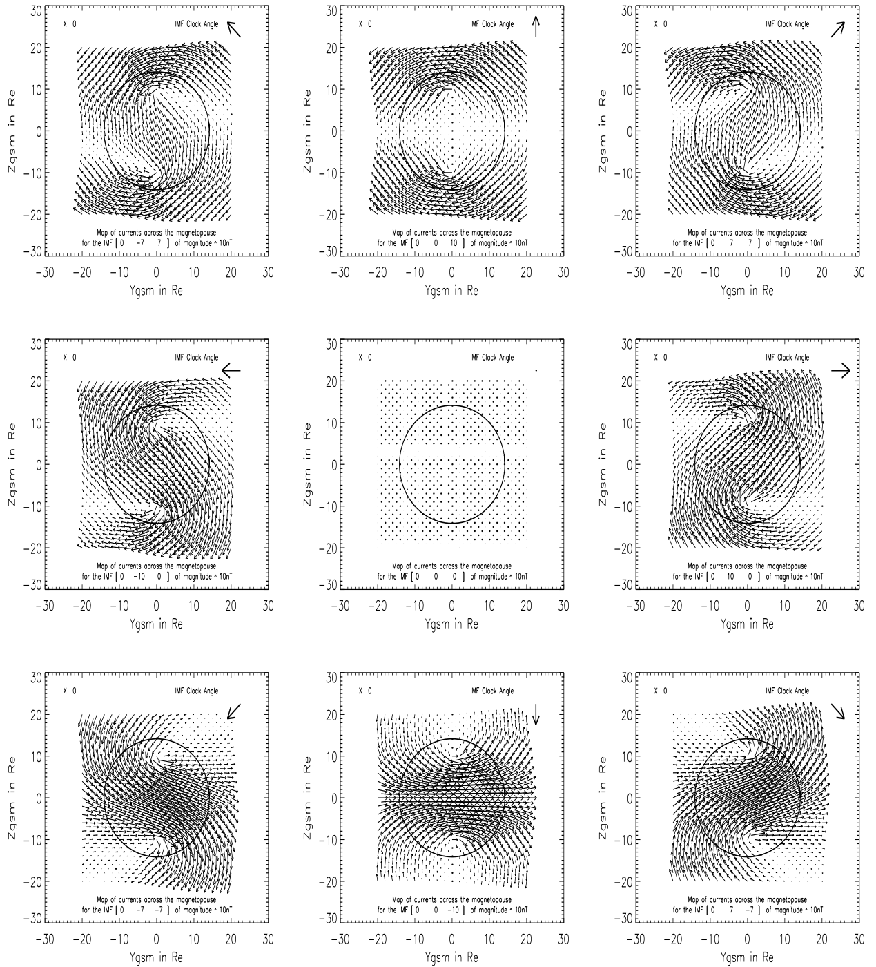
Figure 2.2: Magnetopause current 0X
