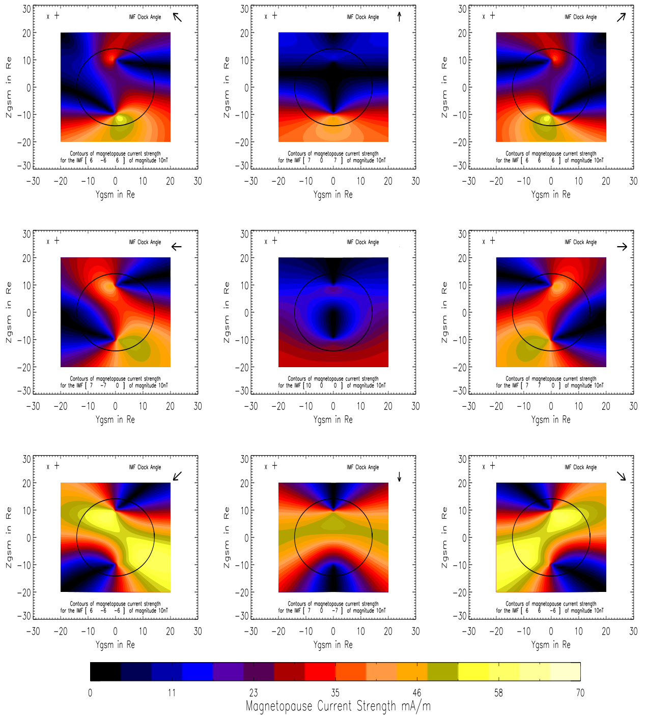
Figure 2.4: Magnetopause current strength contours +X
