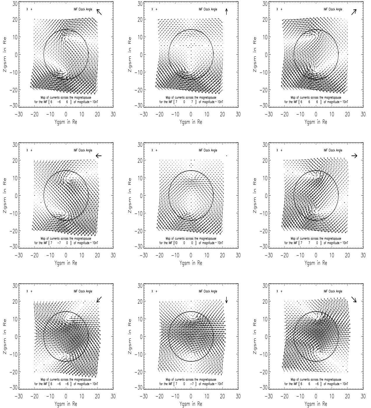
Figure 2.1: Magnetopause current +X
