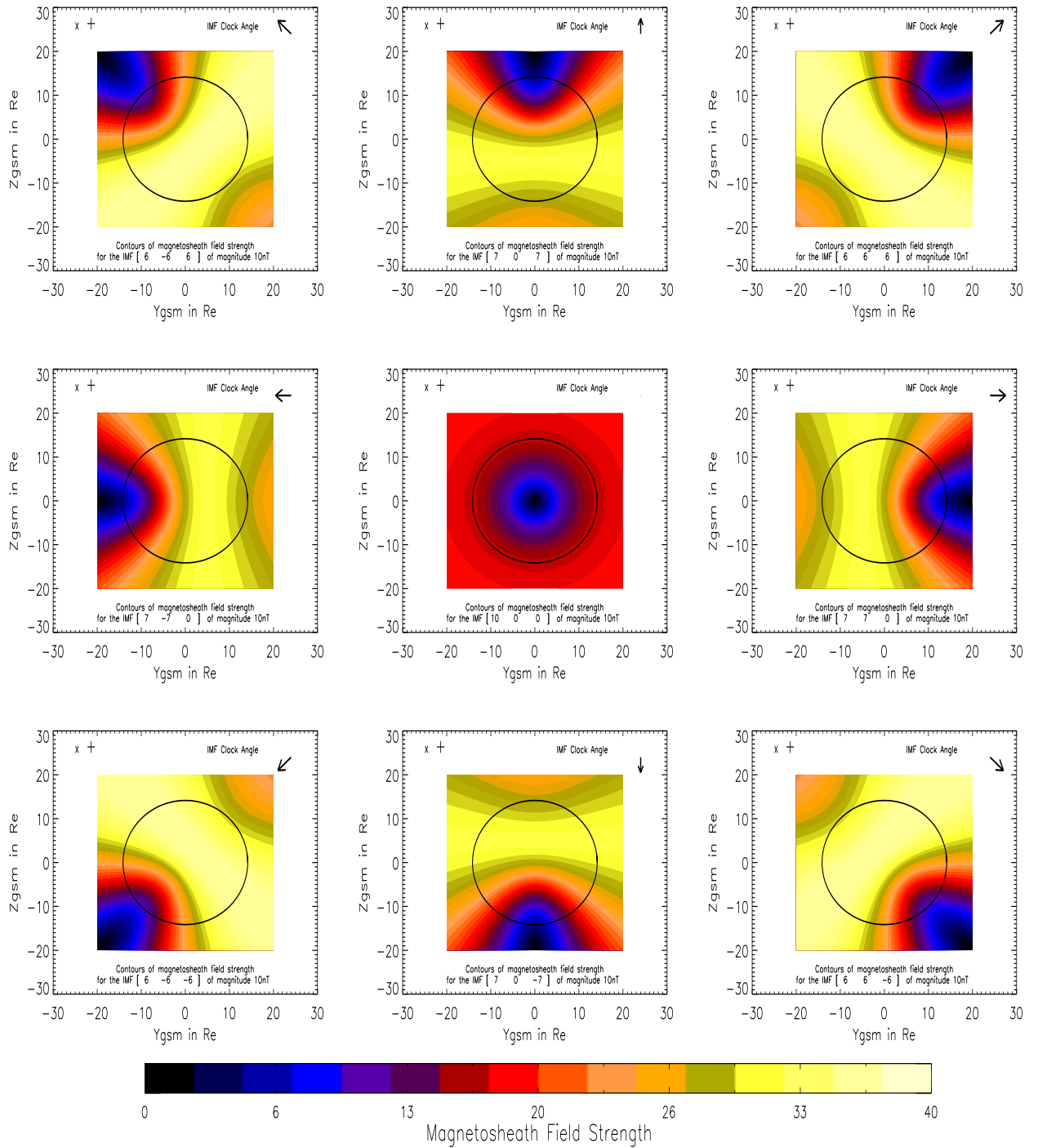
Figure 1.4: Magnetosheath field strength contours -X
