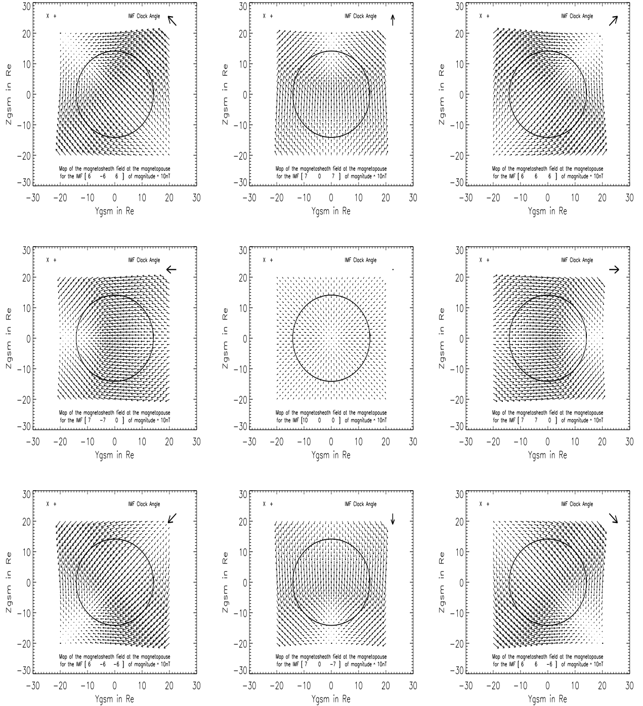
Figure 1.1: Magnetosheath field +X
