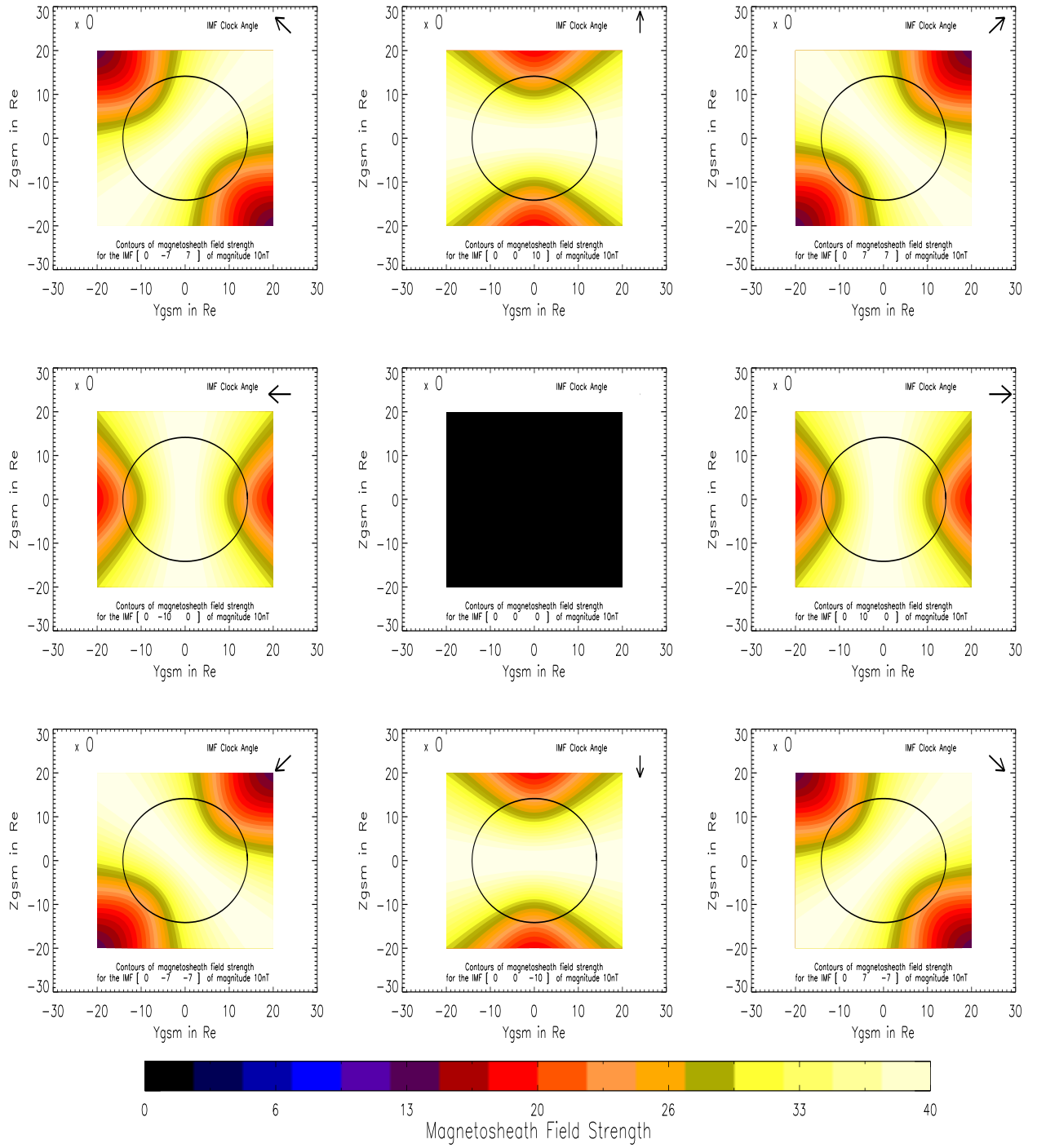
Figure 1.5: Magnetosheath field strength contours OX
