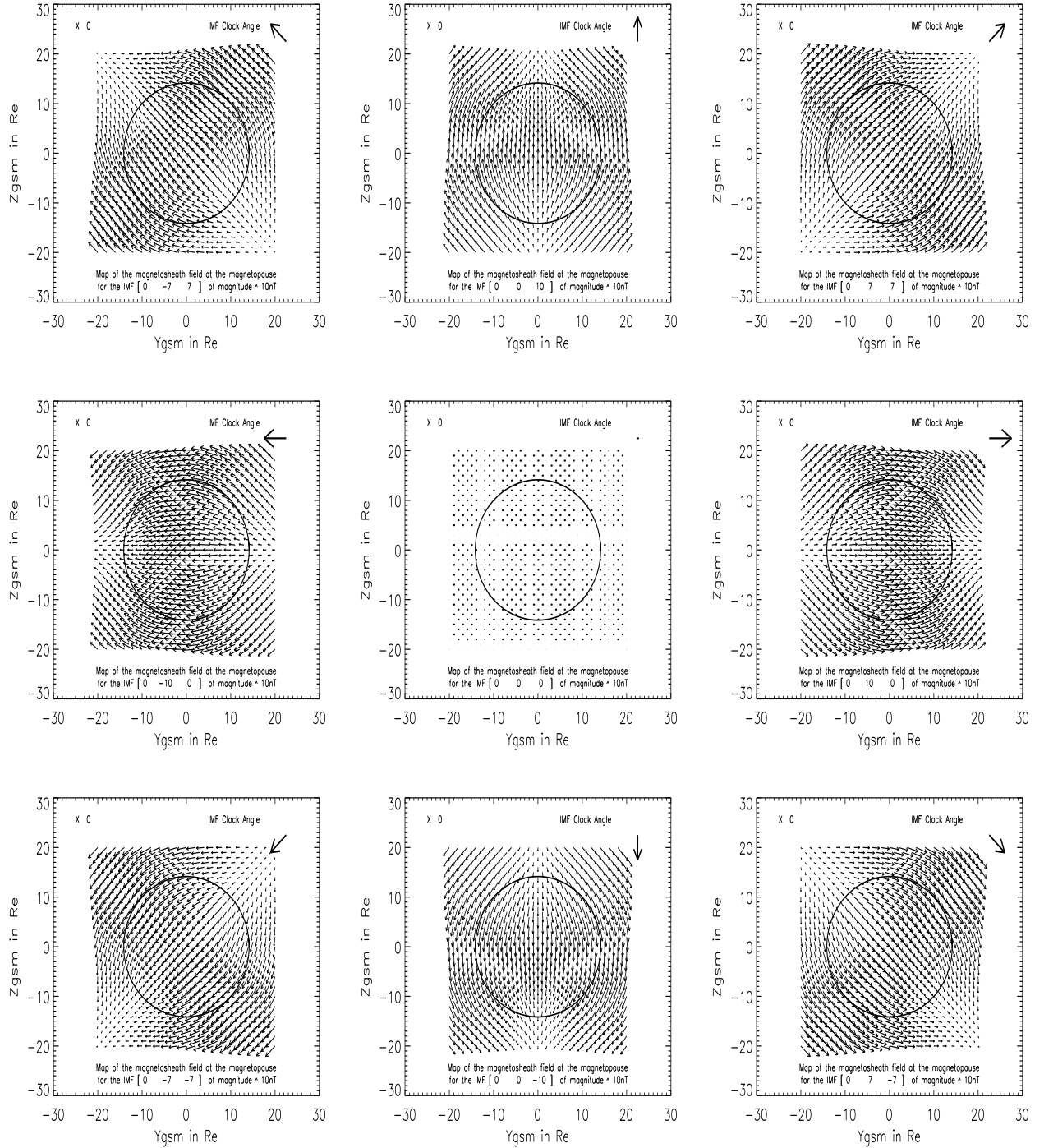
Figure 1.2: Magnetosheath field OX
