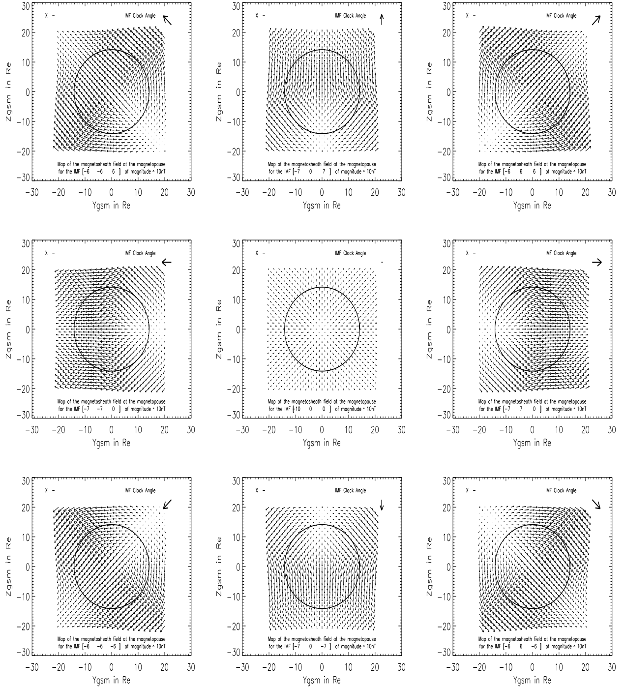
Figure 1.3: Magnetosheath field -X
