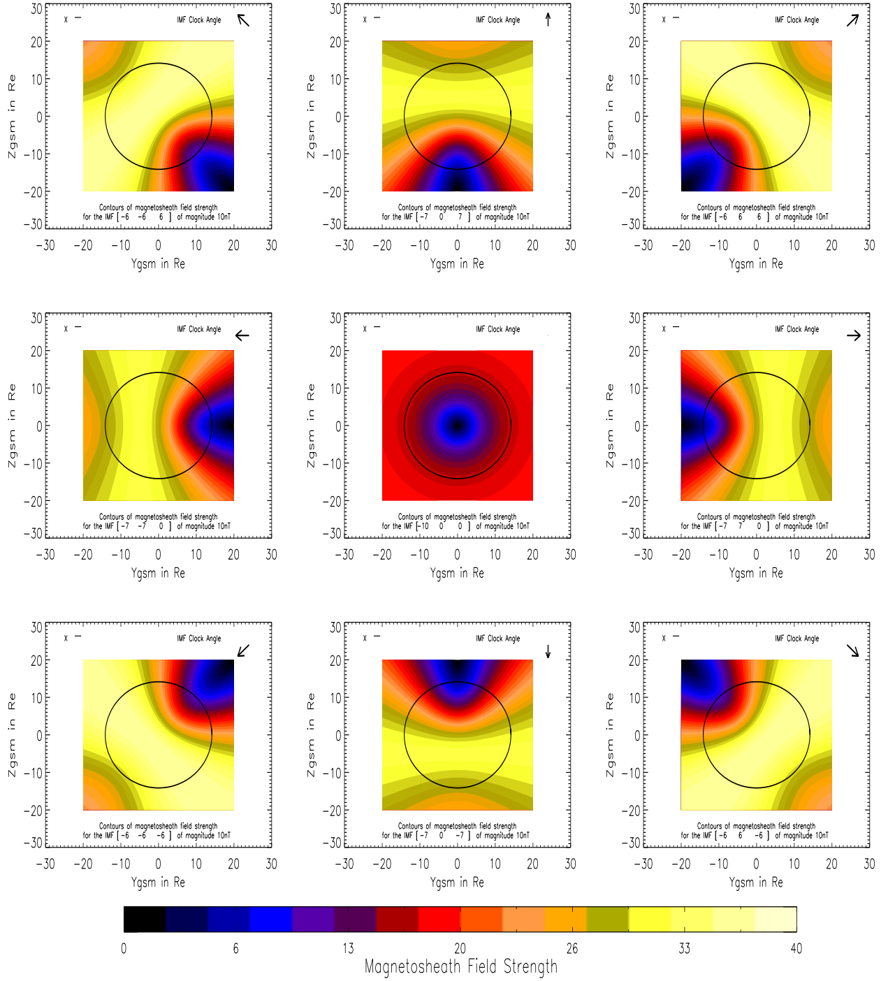
Figure 1.6: Magnetosheath field strength contours +X
